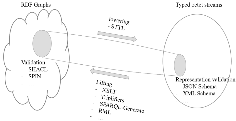
Figure 1: Illustration of an RDF Presentation, pairing RDF Graphs and typed octet stream.
